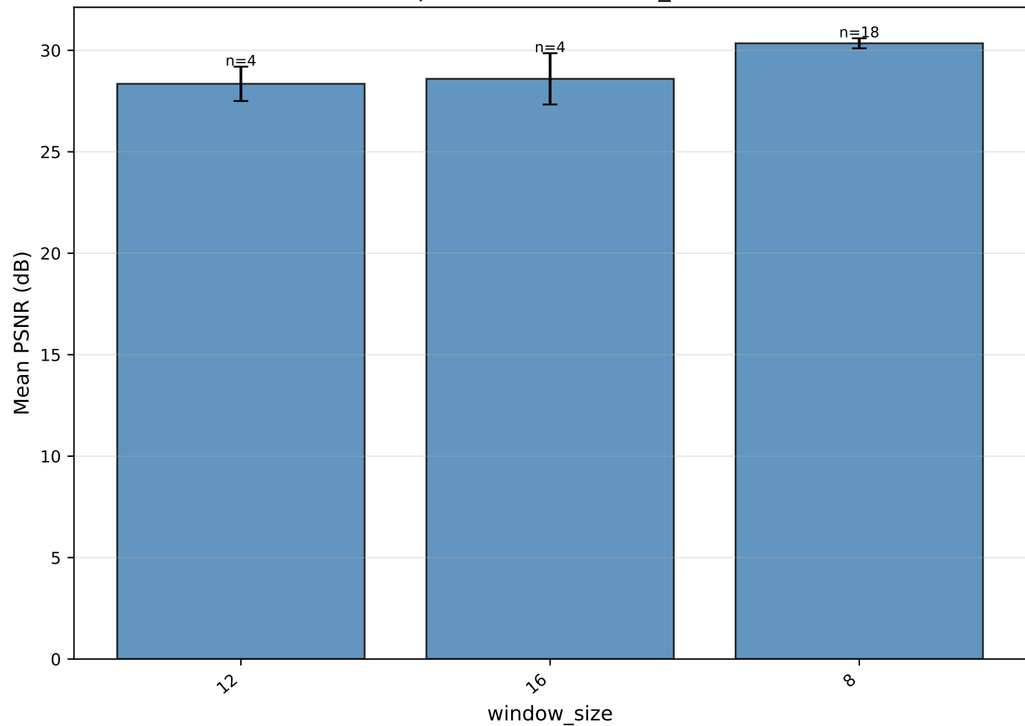
Mean PSNR per value of window_size — SwinT
